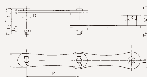
SAV Type Stainless Chain
