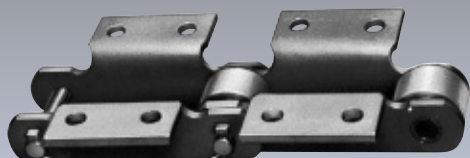
K-type Attachment
