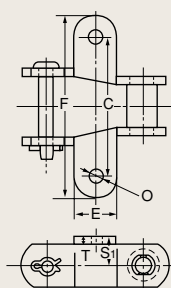
Type 5 Chain
