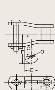
Type 7 Chain
