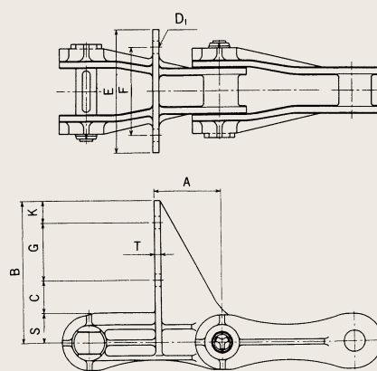
SF4 Attachment
