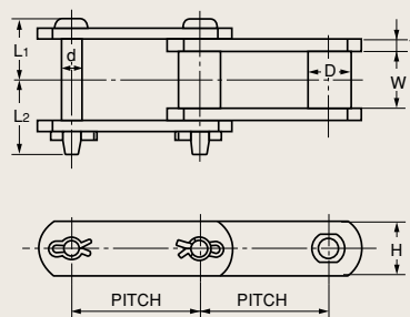
Type 2 Chain
