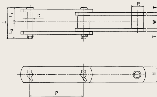
S roller type
