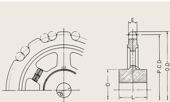
● Sprocket for Combination Chains
