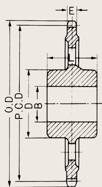
● Sprockets for 710 Pintle Chains
