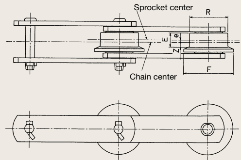
F roller type
