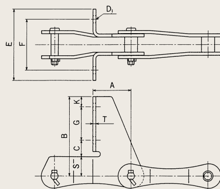
SF4 Attachment
