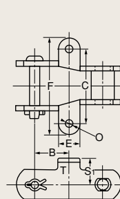
Type 6 Chain
