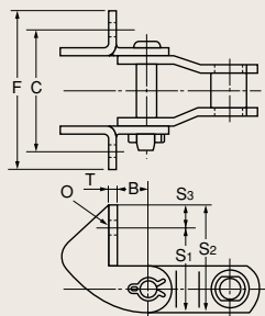
Type 4 Chain
