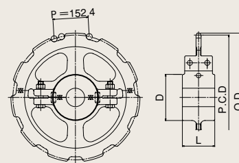
Split type
