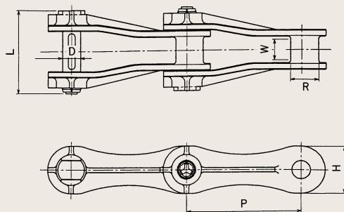
HEP 720S Plastic Chain
